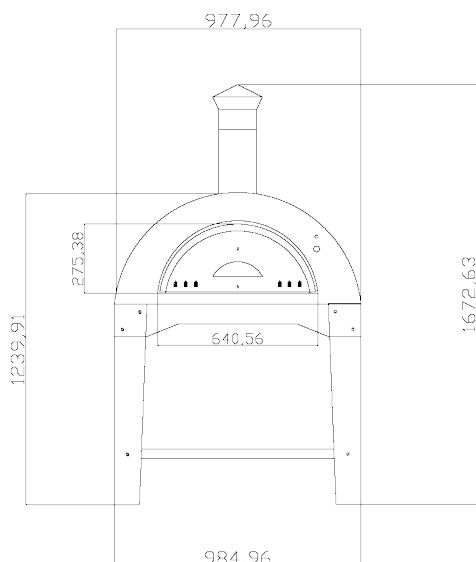
Όψη/ Front view
